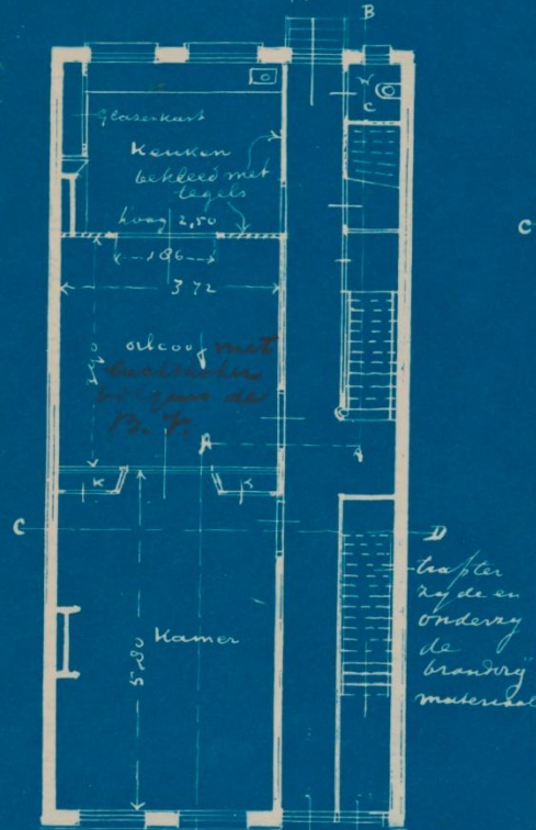
Begane grond Stroomplan
